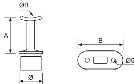
APOYO TUBO RECTO HANDRAIL SUPPORT SUPPORT TUBE
