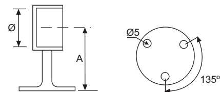
SOPORTE TERMINAL RECTO STRAIGHT HANDRAIL SUPPORT "END" SUPPORT TERMINAL MUR DROIT
