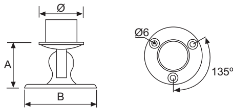
SOPORTE RÓTULA ÁNGULO VARIABLE ADJUSTABLE ROUND BASE PLATE SUPPORT EMBASE BOULE ORIENTABLE
