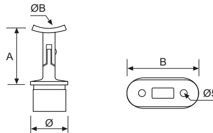
APOYO ÁNGULO VARIABLE ADJUSTABLE HANDRAIL SUPPORT SUPPORT ORIENTABLE
