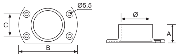
BASE SEMIESFÉRICA SEMISPHERIC BASE PLATE EMBASE HÉMISPHERIQUE
