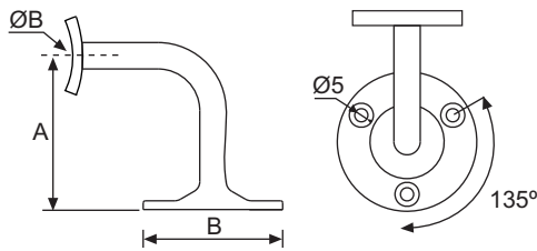
APOYO TUBO 90° 90° BRACKET HANDRAIL SUPPORT SUPPORT MURAL-TUBE 90°
