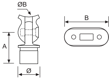
RÓTULA APOYO DE ÁNGULO VARIABLE ADJUSTABLE HANDRAIL SUPPORT-BALL SHAPED SUPPORT BOULE ORIENTABLE
