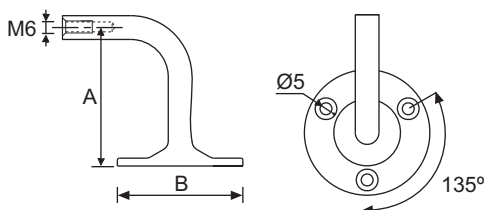
APOYO DE ATORNILLAR 90° SIMPLE 90° WELDING HANDRAIL SUPPORT-THREADED SUPPORT MURAL-TUBE DE VISSER 90°
