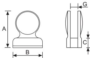
GRAPA PLANA CIRCULAR FLAT GLASS CLAMP-DROP SHAPE PINCE PLATE CIRCULAIRE
