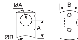
BRIDA CÓNCAVA TERMINAL RADIUSED BAR HOLDER-BLIND SUPPORT TRANSVERSAL BORGNE, CONCAVE
