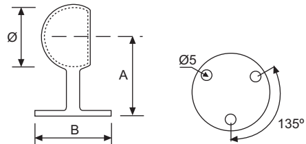
SOPORTE TERMINAL REDONDO BALL HANDRAIL SUPPORT "END" SUPPORT TERMINAL MUR ARRONDI
