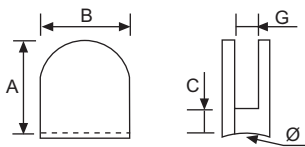
GRAPA CÓNCAVA RADIUSED GLASS CLAMP PINCE CONCAVE
