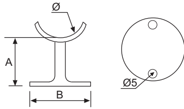
APOYO TUBO A PARED BRACKET HANDRAIL SUPPORT SUPPORT MURAL-TUBE
